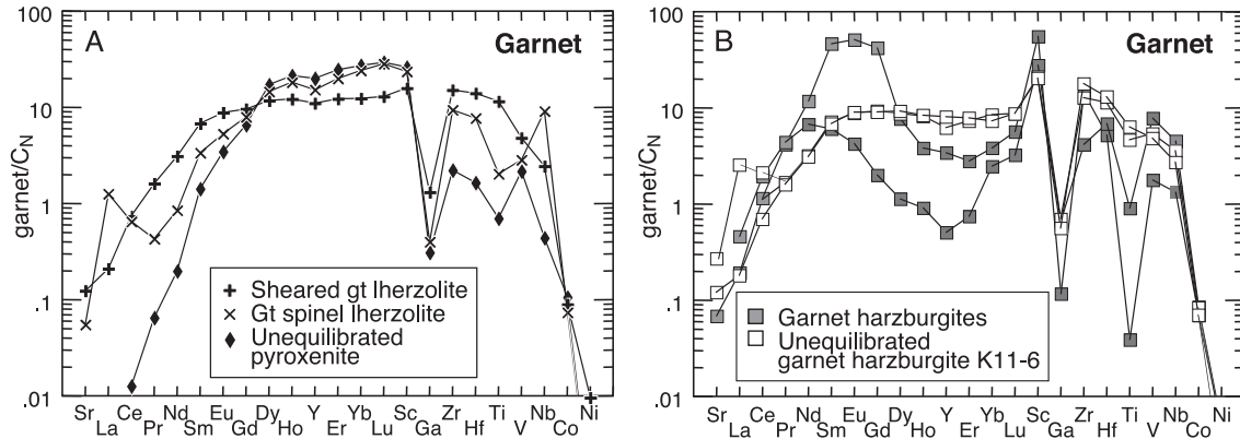
Fig. 5. Extended trace-element patterns in garnet. C_N denotes normalisation to chondrite of McDonough and Sun (1995).
