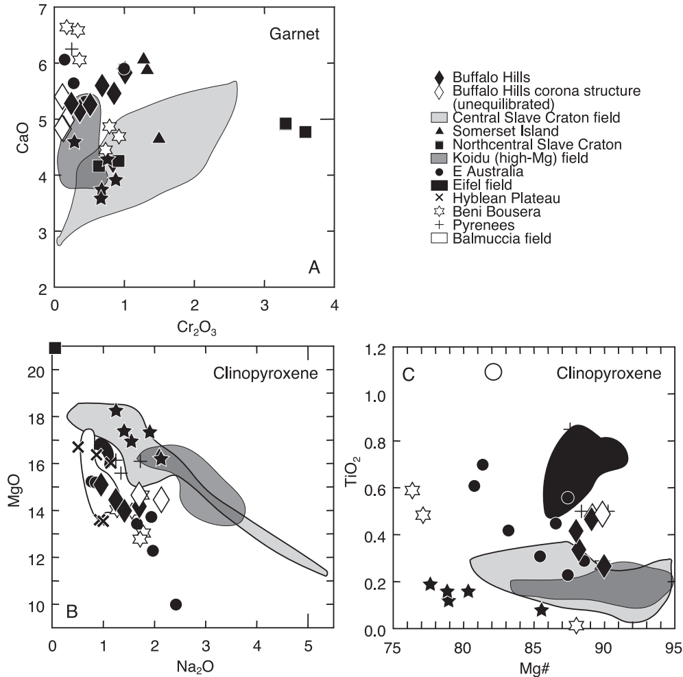
Fig. 15. (A) \text{Cr}_2\text{O}_3 against CaO in garnet, (B) \text{Na}_2\text{O} against MgO in cpx and (C) Mg# against \text{TiO}_2 in cpx in pyroxenites from Buffalo Hills. Shown for comparison are pyroxenite xenoliths and pyroxenites in peridotite massifs (Beni Bousera, Morocco: Komprobst, 1969 ; Pyrenées: Bodinier et al., 1987 ; Balmuccia: Rivalenti et al., 1995 ; Eastern Australia: O'Reilly and Griffin, 1995 ; Hyblean Plateau, Sicily: Nimis and Vannucci, 1995 ; Eifel volcanic fields, Germany: Witt-Eickschen et al., 1998 ; other references as in Fig. 10 ).
