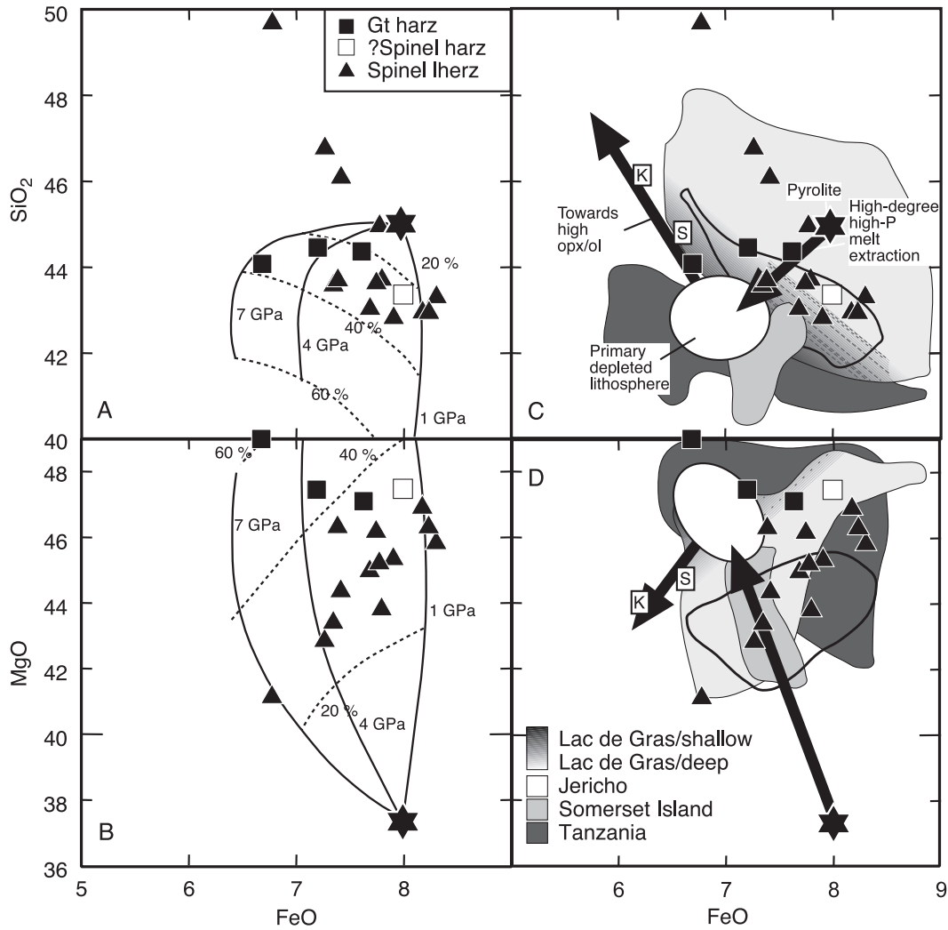
Fig. 9. Whole-rock FeO against (A) SiO 2 and (B) MgO of peridotites from the Buffalo Hills kimberlites (reconstructed from mineral data and modal estimates). (A) and (B) compared to experimental residues of isobaric batch melting at different pressures (solid lines, pressures in GPa) of pyrolite (star) for different degrees of partial melting (hatched lines, percentages; from Walter, 1999); (C, D) partial melting trend, primary depleted lithosphere, trend towards high opx/ol ratios and average compositions of peridotites from the Kaapvaal craton (K) and Siberia (S) (from Walter, 1999); also shown are fields for peridotites from Lac de Gras (central Slave craton: Pearson et al., 1999; unpublished data), Jericho (north-central Slave craton: Kopylova et al., 1999), Somerset Island (Schmidberger and Francis, 1999) and Tanzania (Lee and Rudnick, 1999).
