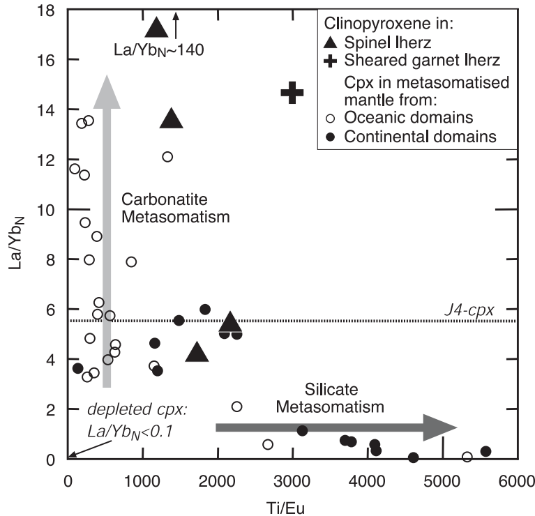
Fig. 13. Ti/Eu against La/Yb N in cpx from Buffalo Hills. Shown for comparison are clinopyroxenes in carbonatite and silicate melt metasomatised samples from oceanic and continental mantle (from Coltorti et al., 1999). Depleted cpx from Norman (1998), primitive J4 cpx of Jagoutz and Spettel (in Stachel et al., 1998); chondrite of McDonough and Sun (1995).
